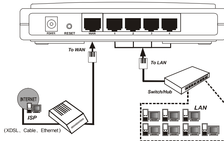
Figure 3-1 Hardware Installation of the TL-R402M Cable/DSL Router
